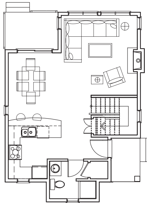
MAIN FLOOR
